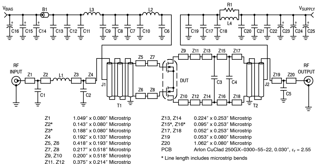
Figure 2. MRF6VP2600HR6 Test Circuit Schematic
