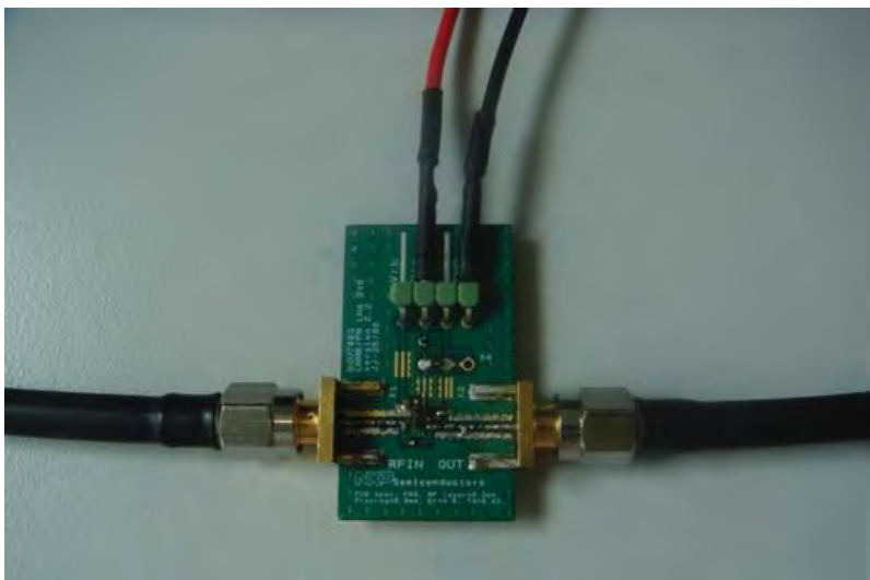
Fig 6. Evaluation board and connectors
