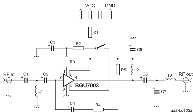
Fig 3. Circuit diagram of the evaluation board
