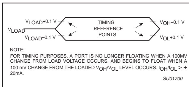
Figure 8. Float Waveform
