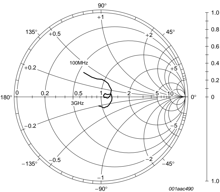
Fig 2. Output reflection coefficient ( s_{22} ); typical values
