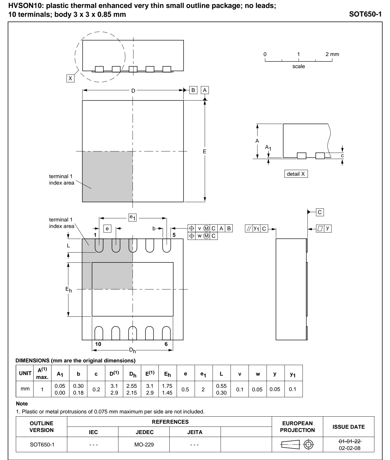
Fig 13. Package outline SOT650-1 (HVSON10)
