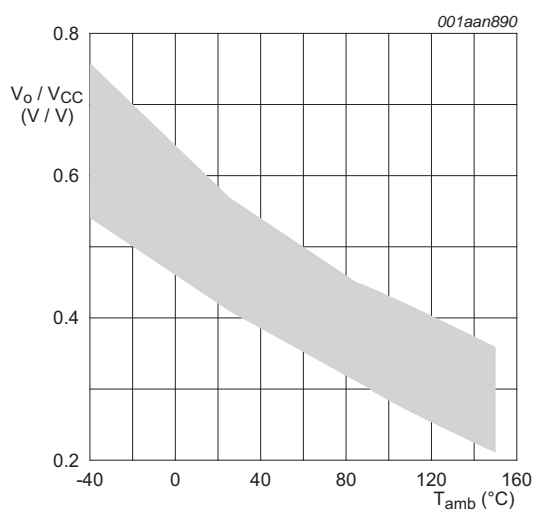
Fig 6. Output signal peak-to-peak amplitude with pin TCC_EN connected to ground
