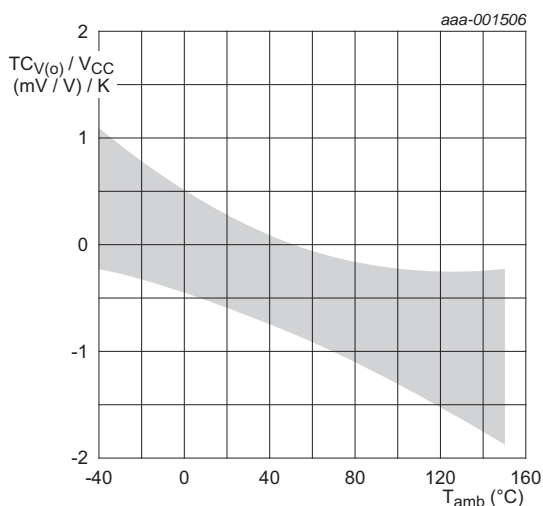
Fig 7. TC of output signal peak-to-peak amplitude with pin TCC_EN connected to V_{CC}
