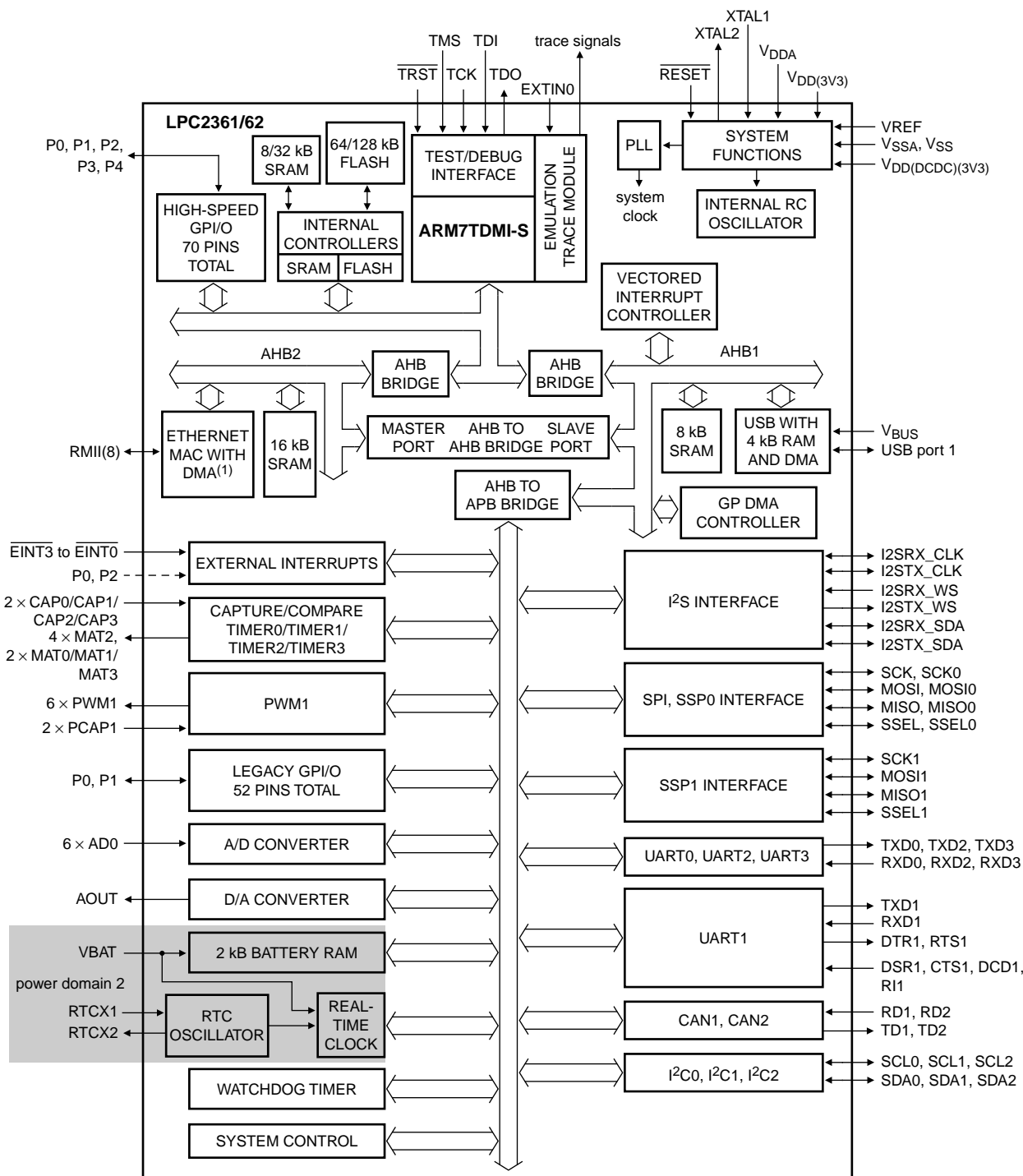
Fig 1. LPC2361/2362 block diagram
