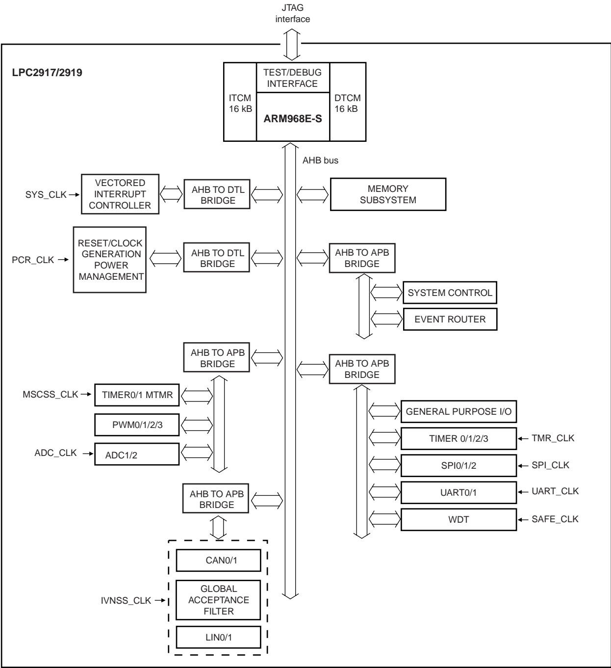
Fig 3. LPC2917/19 block diagram, overview of clock areas
