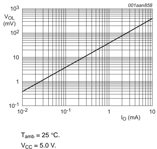
Fig 9. LOW-level output voltage versus output current
