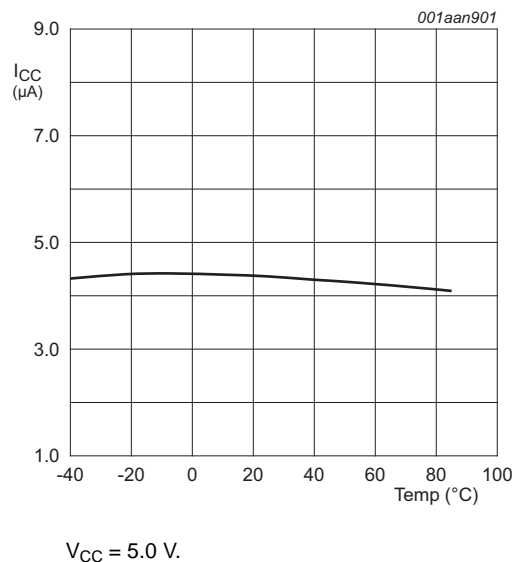
Fig 6. Supply current versus temperature (per comparator)
