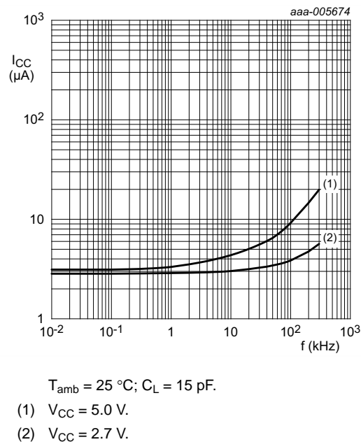
Fig 7. Supply current versus output transition frequency (per comparator)
