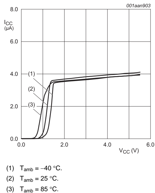
Fig 8. Supply current versus supply voltage (per comparator)
