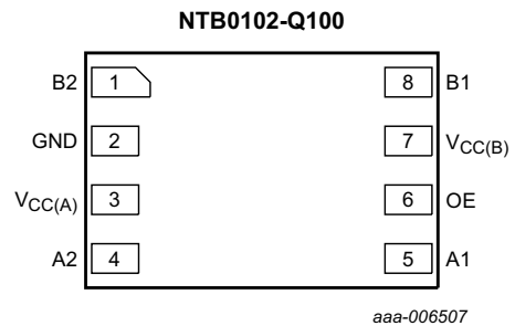
Fig 3. Pin configuration SOT996-2 (XSON8)
