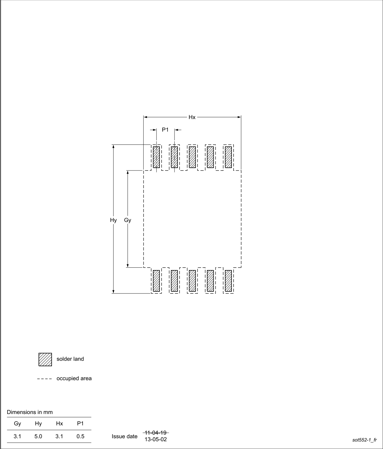
Fig 23. PCB footprint for SOT552-1 (TSSOP10); reflow soldering
