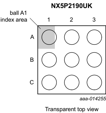
Fig 3. Pin configuration WLCSP9 package
