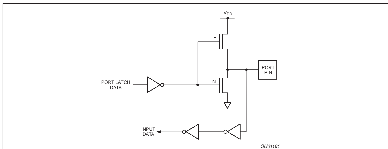
Figure 12. Push-Pull Output
