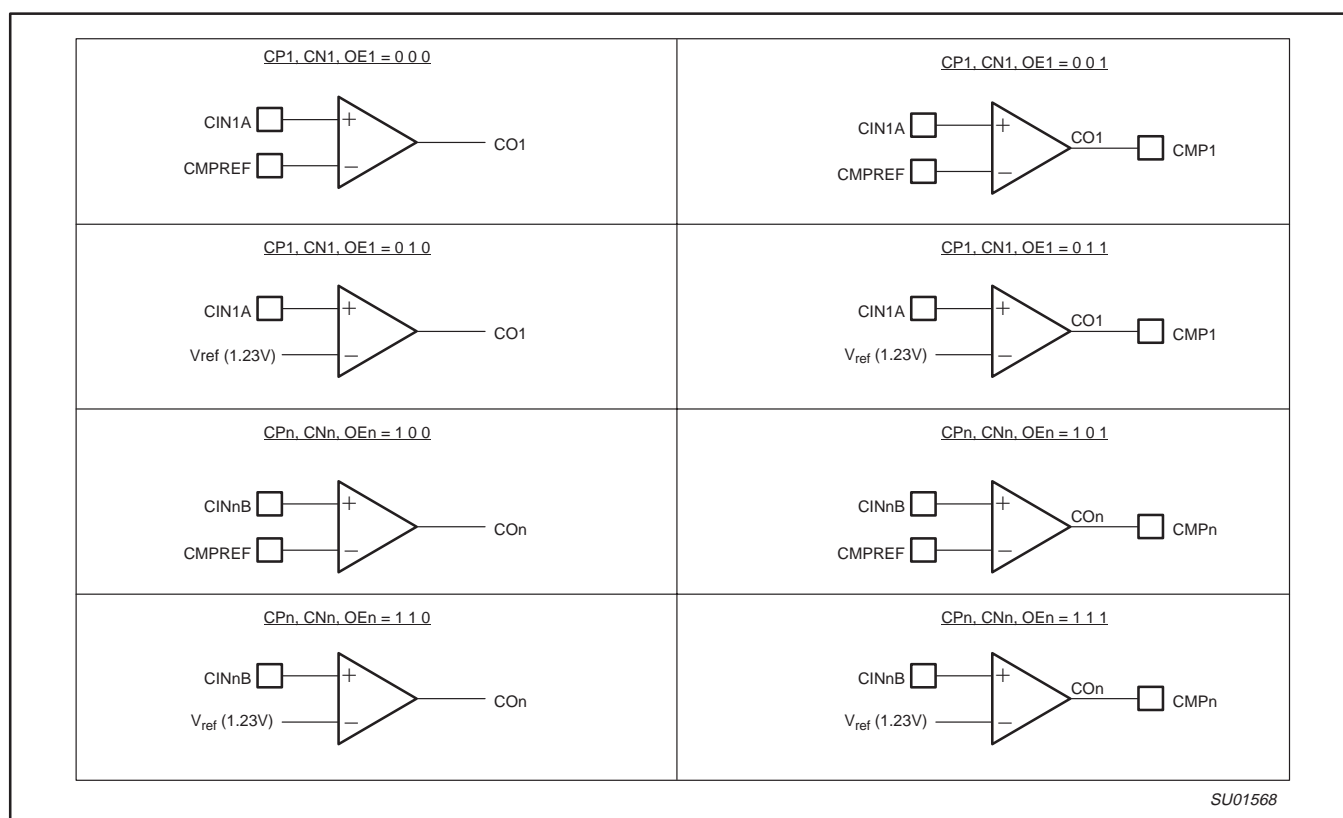
Figure 4. Comparator Configurations
