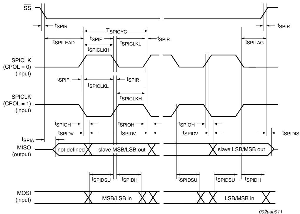
Fig 37. SPI slave timing (CPHA = 1)
