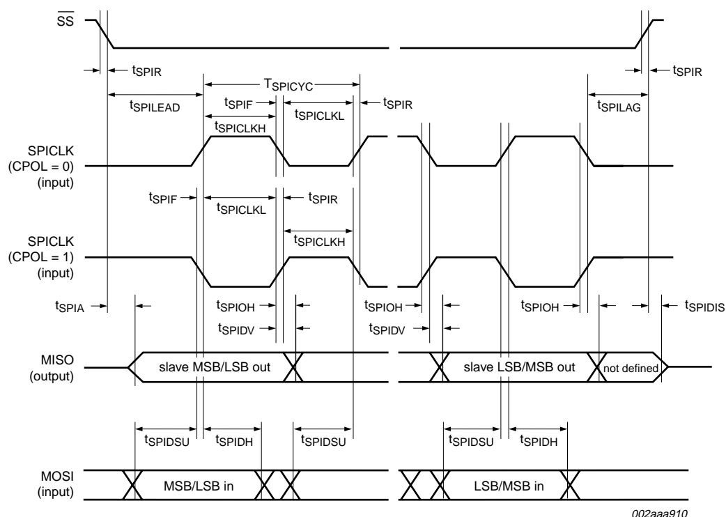
Fig 36. SPI slave timing (CPHA = 0)
