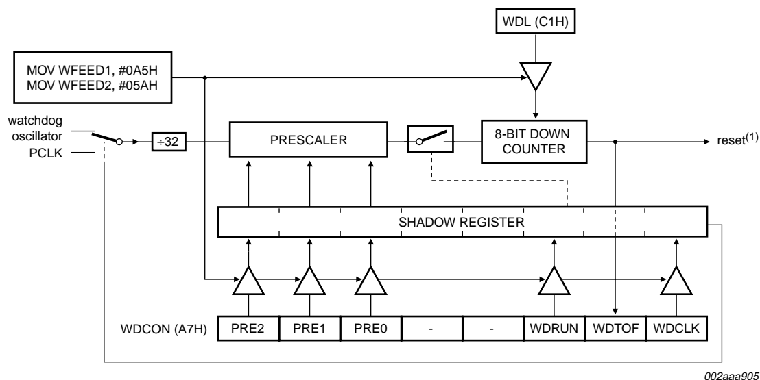
Fig 23. Watchdog timer in Watchdog mode (WDTE = '1')
