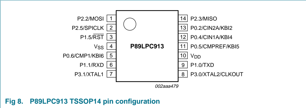
Fig 7. P89LPC912 TSSOP14 pin configuration
