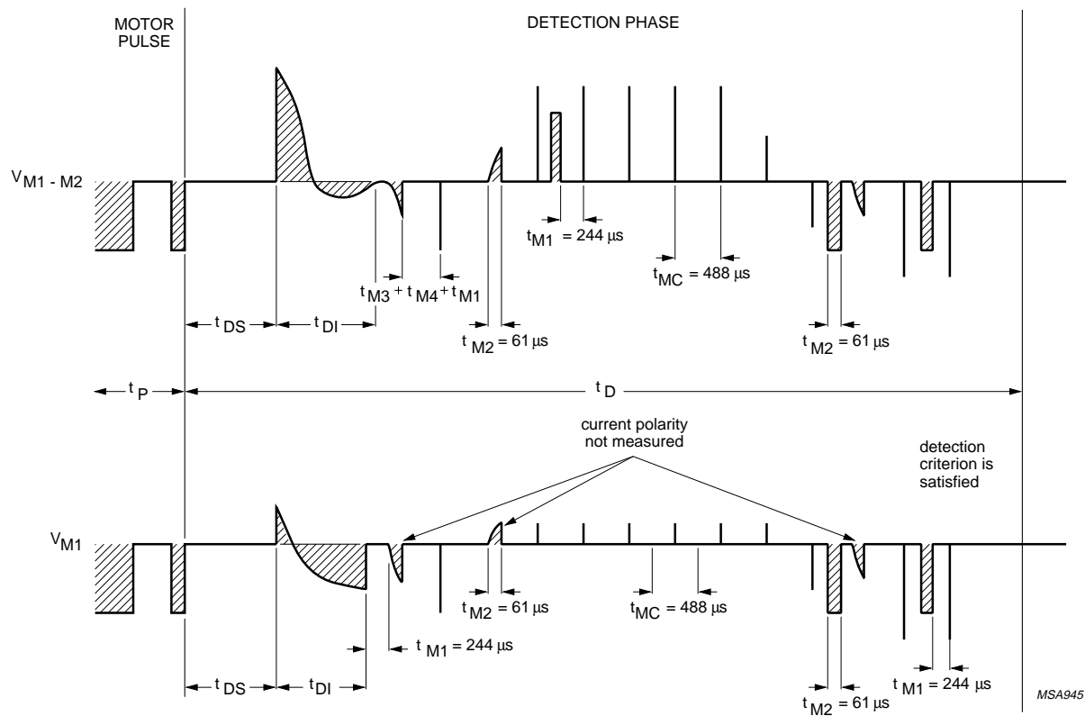
Fig.7 Detection phase of the current waveform in Fig.6.
