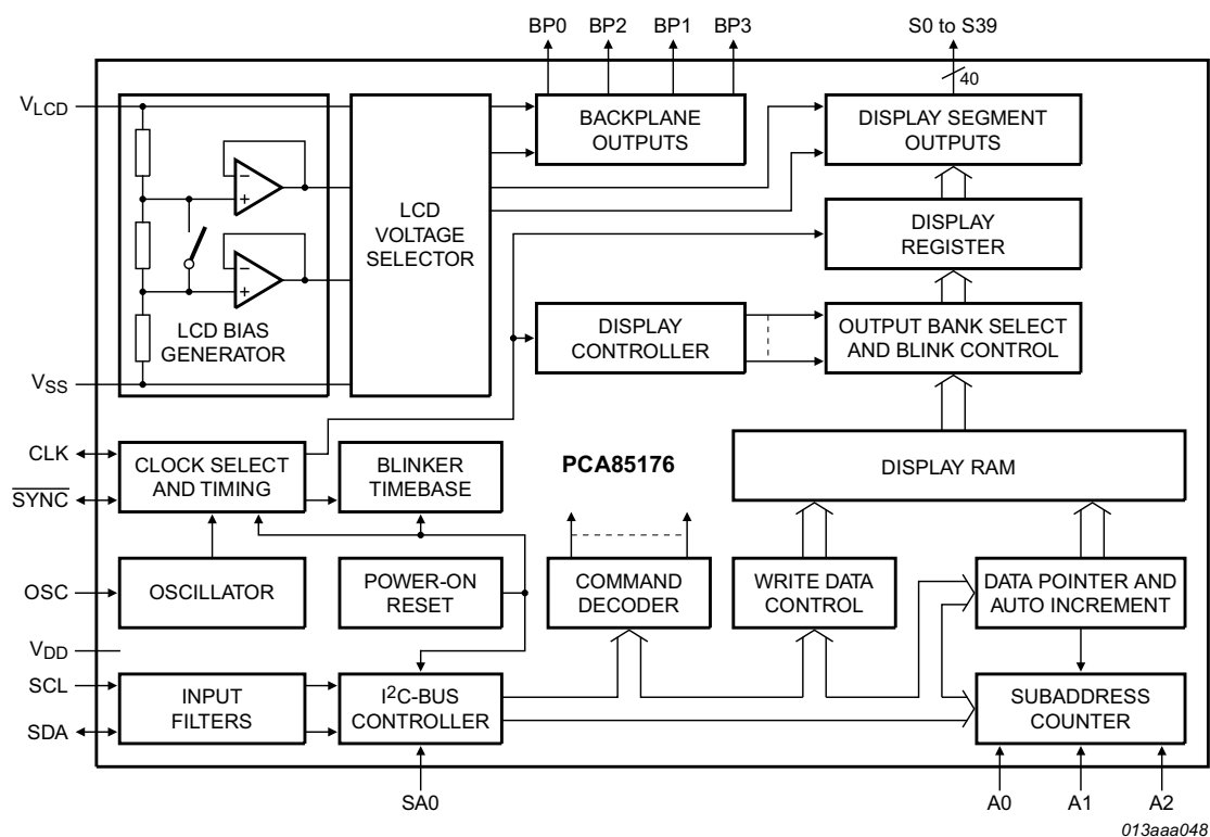
Fig 1. Block diagram of PCA85176
