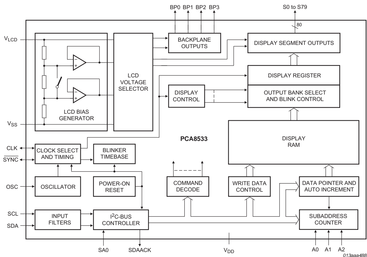
Fig 1. Block diagram of PCA8533
