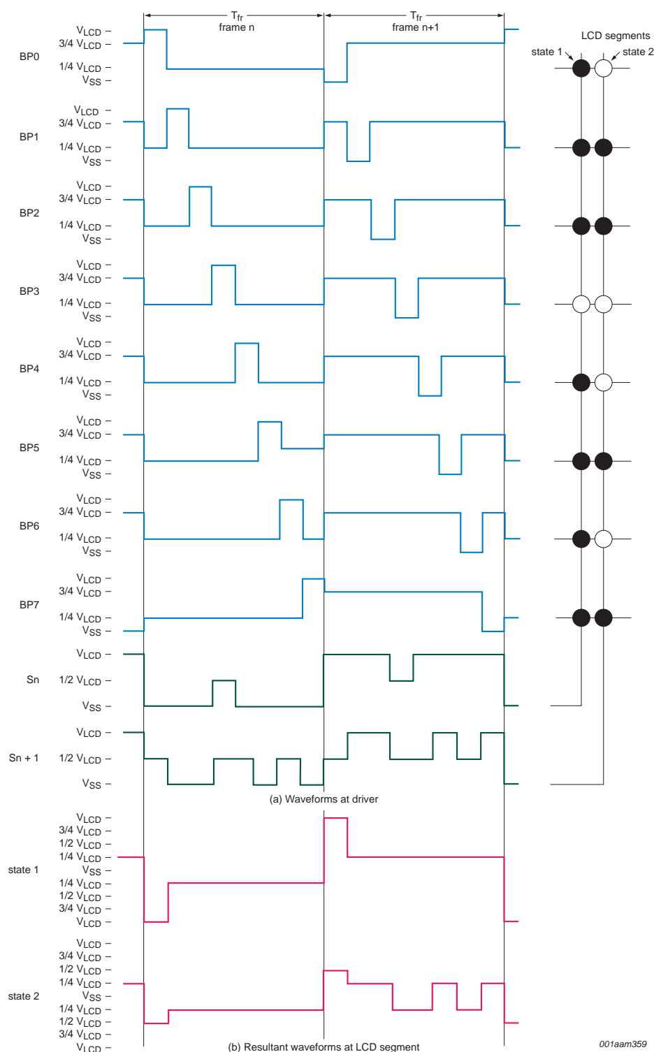
Fig 19. Waveforms for 1:8 multiplex drive mode with bias 1/4 and frame inversion
