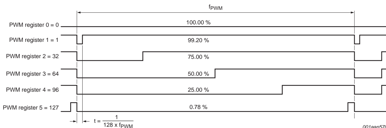
Fig 30. PWM example waveforms for PWMI = 1
