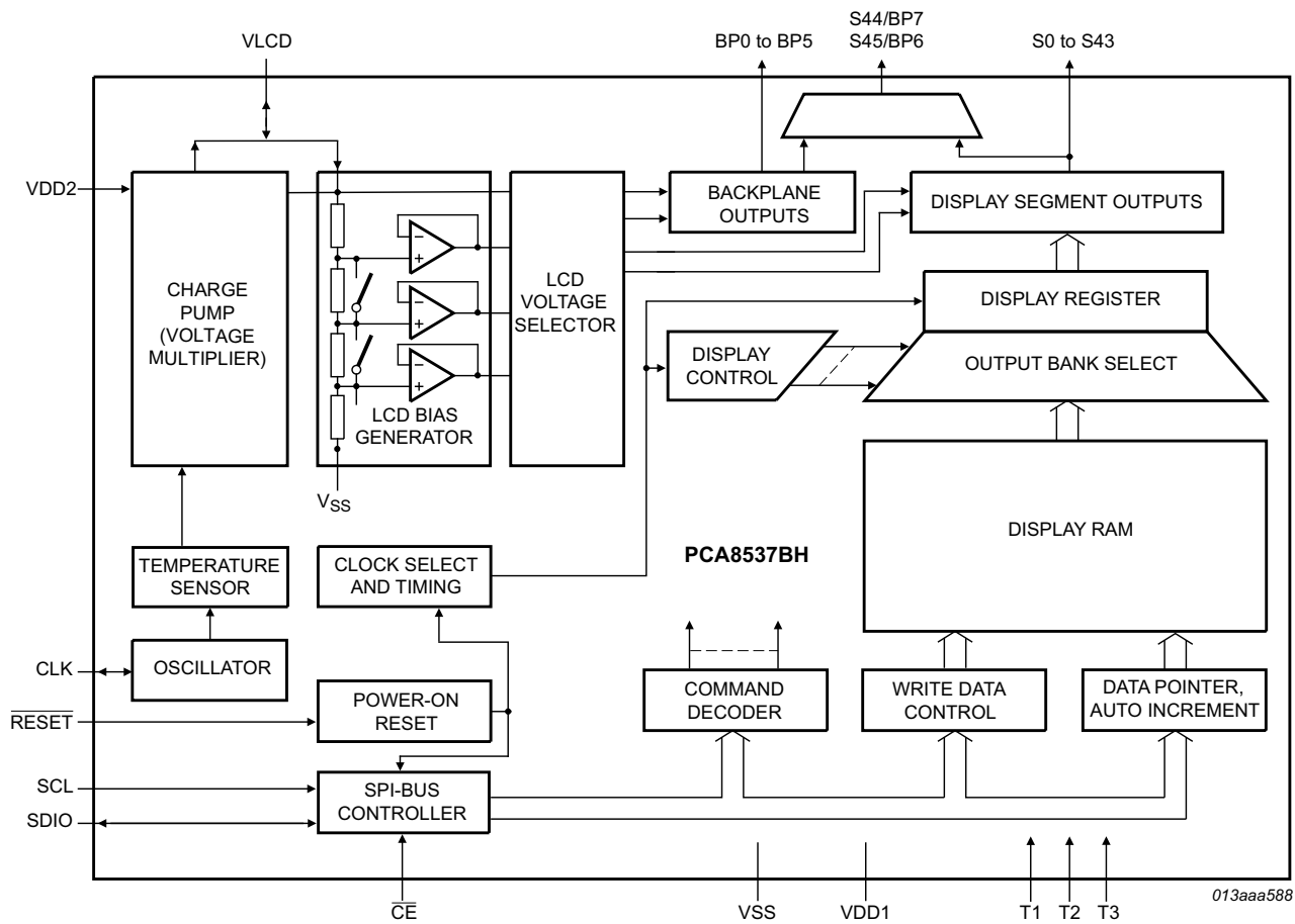
Fig 2. Block diagram of PCA8537BH
