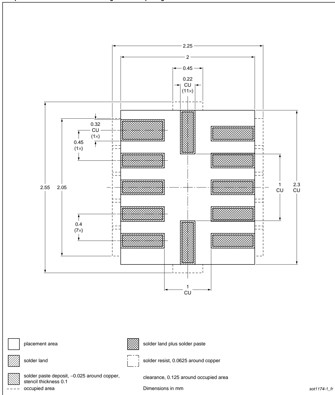
Fig 30. PCB footprint for SOT1174-1 (XQFN12); reflow soldering
