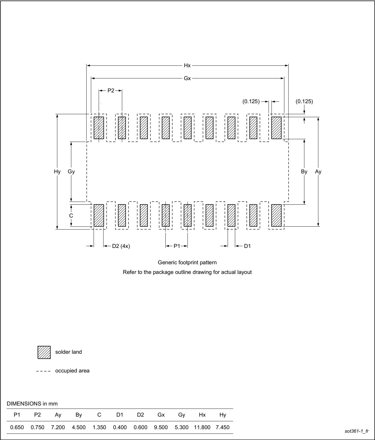
Footprint information for reflow soldering of TSSOP28 package SOT361-1
