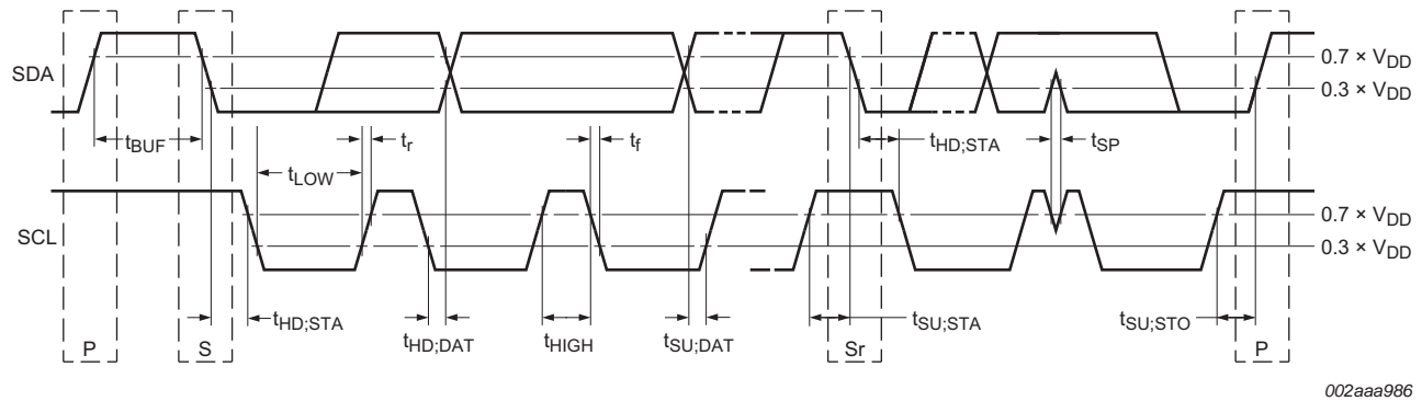
Fig 26. Definition of timing
