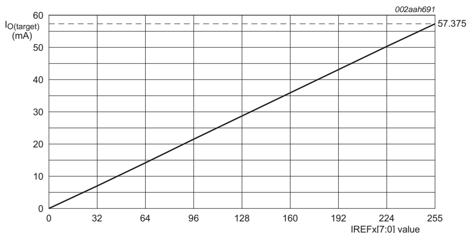
Fig 11. I_{O(target)} versus IREF x value with R_{ext} = 1 \text{ k}\Omega
