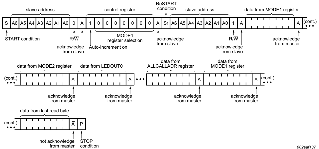
Fig 22. Read all registers using the Auto-Increment feature
