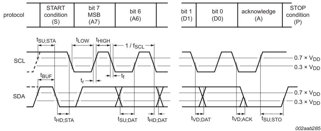
Fig 27. I 2 C-bus timing diagram
