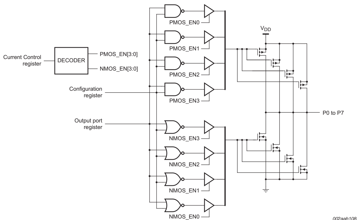
Fig 15. Simplified output stage
