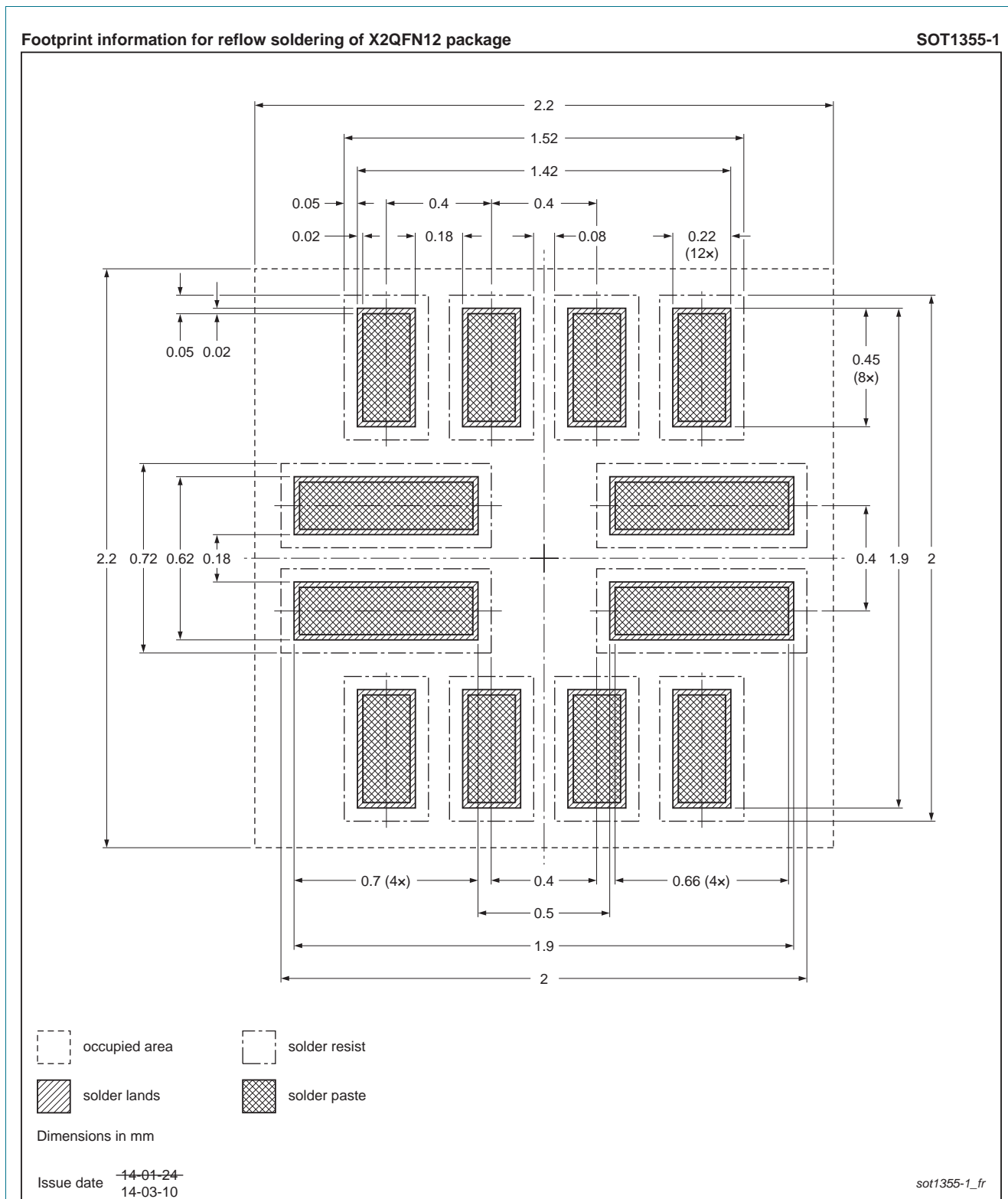
Fig 17. PCB footprint for SOT1355-1 (X2QFN12); reflow soldering
