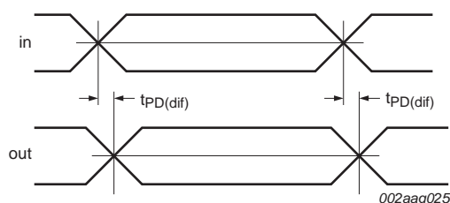
Fig 6. Propagation delay
