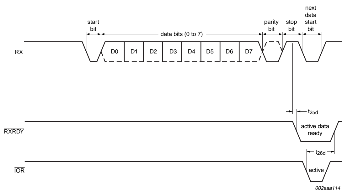
Fig 14. Receive ready timing in non-FIFO mode
