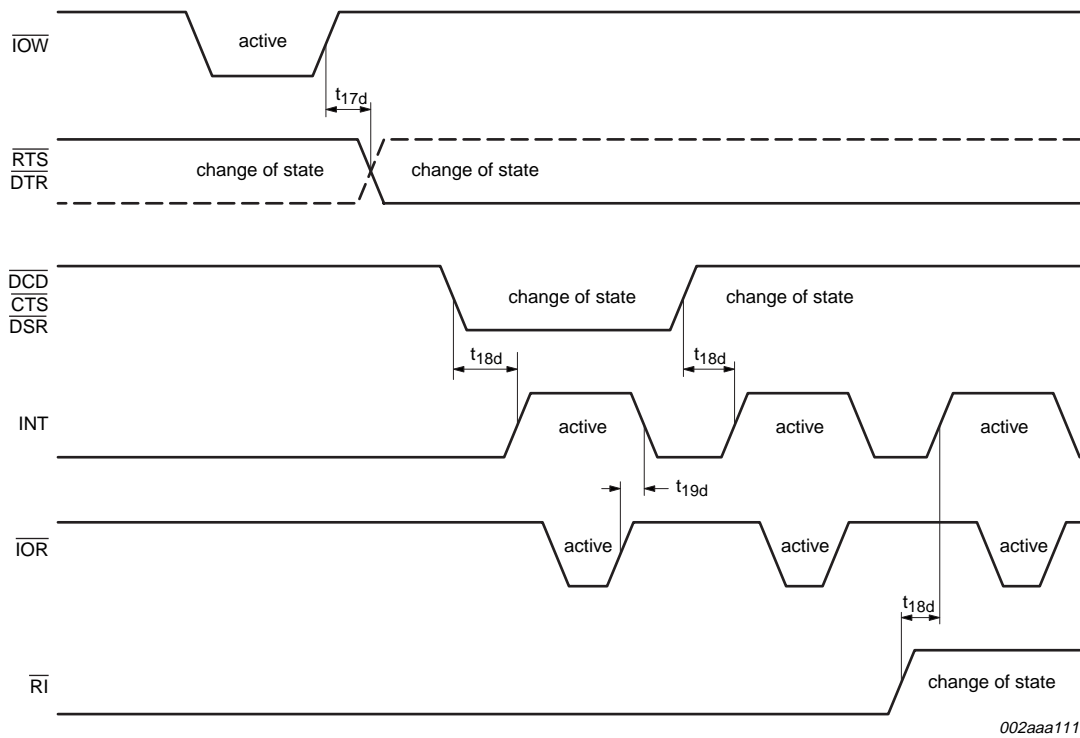
Fig 11. Modem input/output timing
