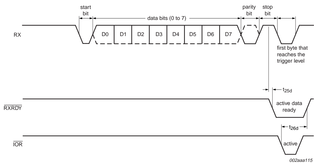
Fig 15. Receive ready timing in FIFO mode
