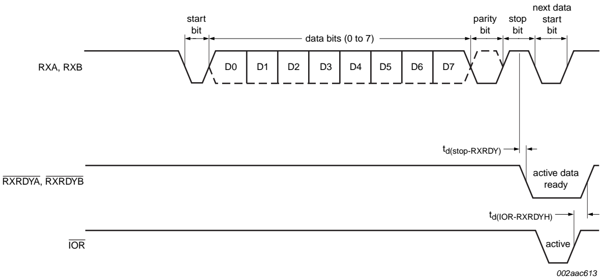
Fig 20. Receive ready timing in non-FIFO mode (16 mode)
