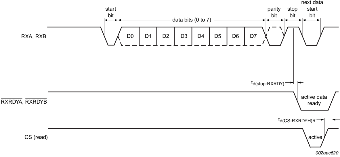
Fig 21. Receive ready timing in non-FIFO mode (68 mode)
