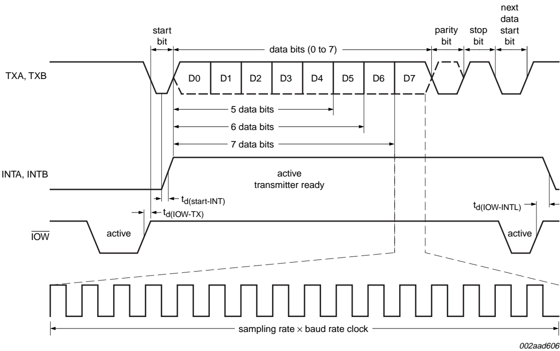
Fig 13. Transmit timing
