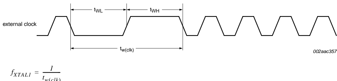
Fig 24. External clock timing
