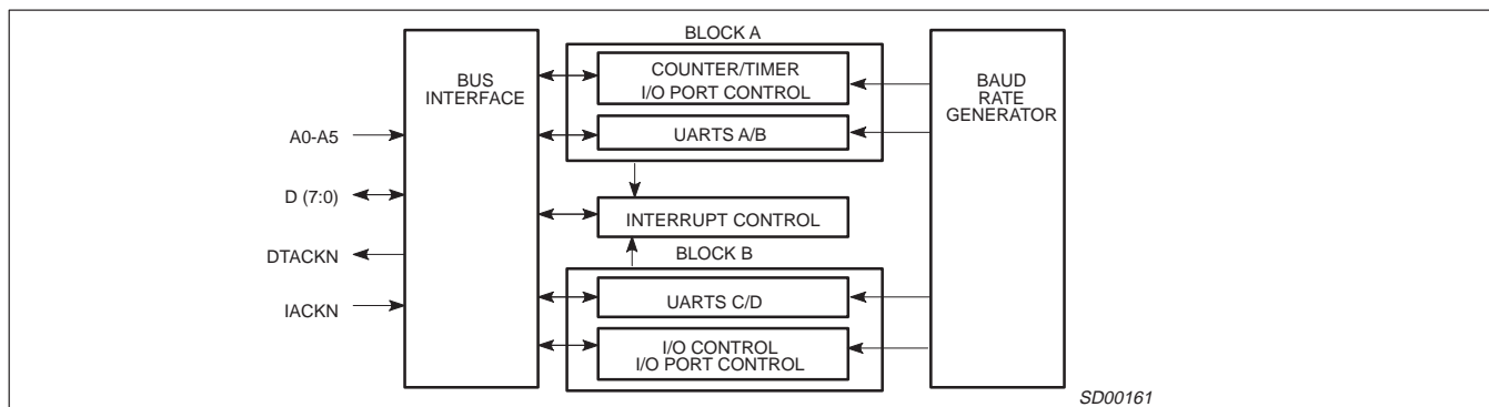
Figure 3. Channel Architecture
