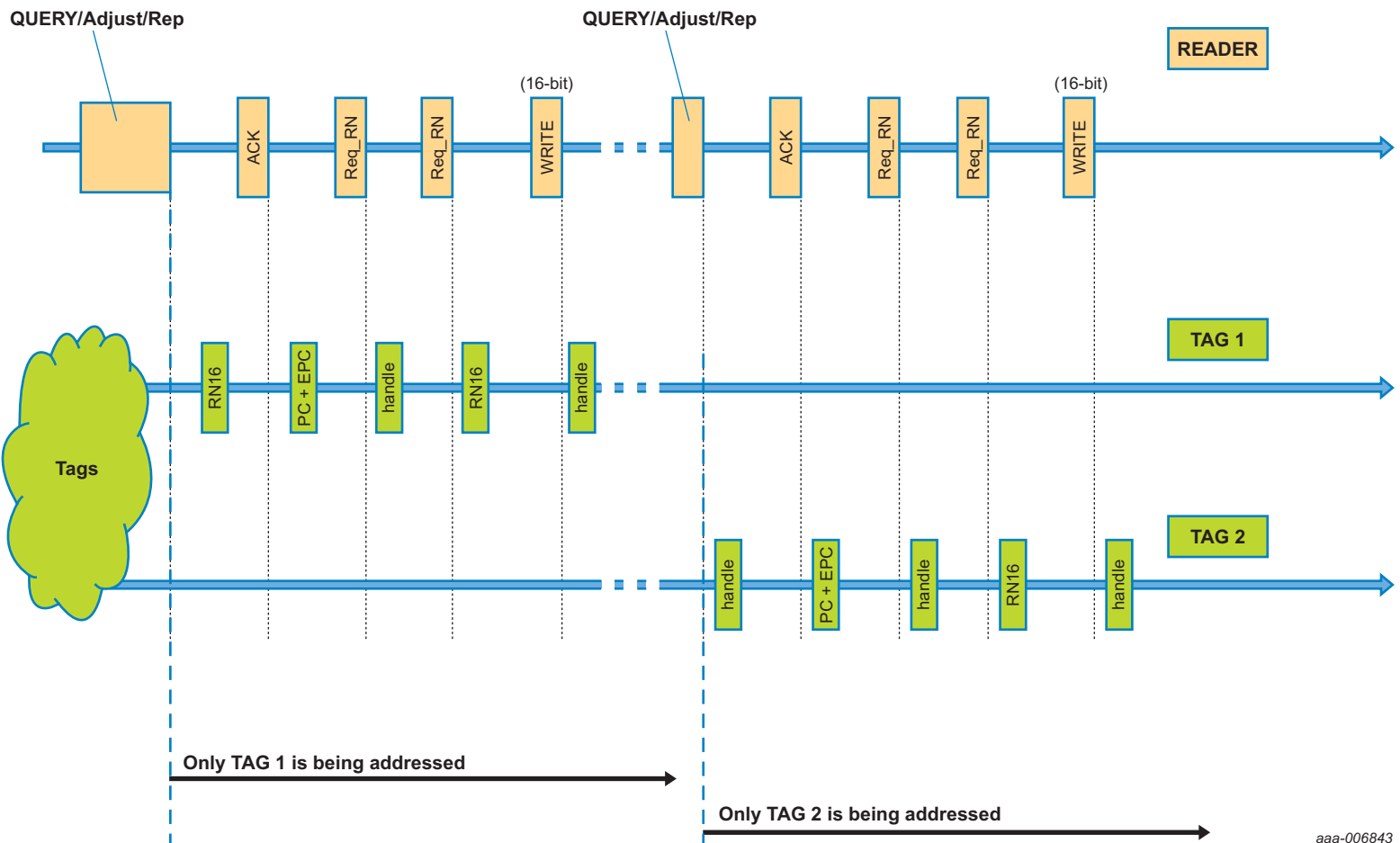
Fig 8. Example of 16-bit Write command with standard EPC Gen 2 commands
