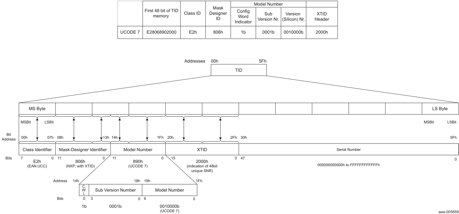
Fig 7. UCODE 7 TID memory structure
