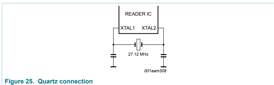
Figure 25. Quartz connection
