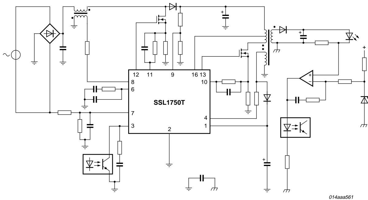
Fig 3. Application circuit
