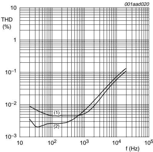
R_L = 4\text{ }\Omega ; 80 kHz measurement filter. (1) P_o = 1\text{ W} . (2) P_o = 10\text{ W} .
