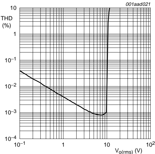
R_L = 100\text{ }\Omega ; 80 kHz measurement filter; f = 1\text{ kHz} .
