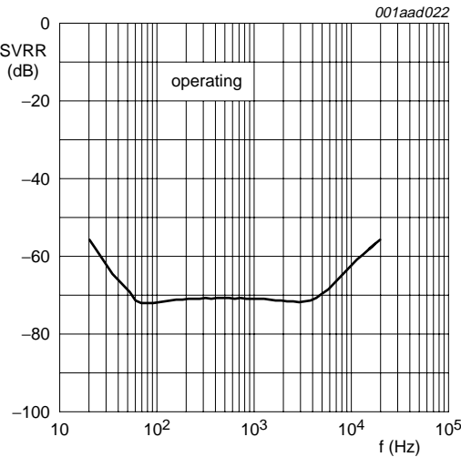
R_s = 1\text{ k}\Omega ; C_{SVR} = 10\text{ }\mu\text{F} .
