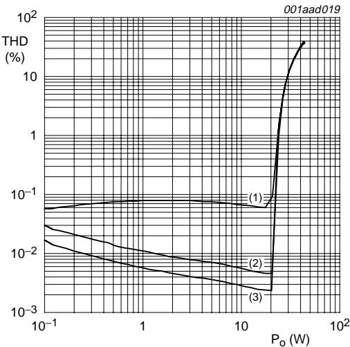
R_L = 4\text{ }\Omega ; 80 kHz measurement filter. (1) f = 10\text{ kHz} . (2) f = 1\text{ kHz} . (3) f = 100\text{ Hz} .
