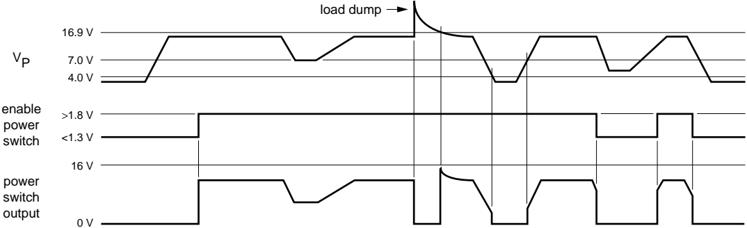
Power switch behaviour
