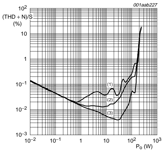
Fig 10. (THD + N)/S as a function of output power; SE configuration with 2 × 3 \Omega load
