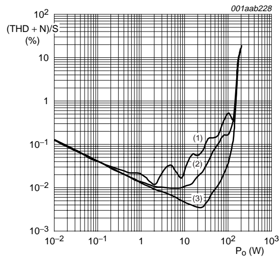
Fig 11. (THD + N)/S as a function of output power; SE configuration with 2 × 4 \Omega load
