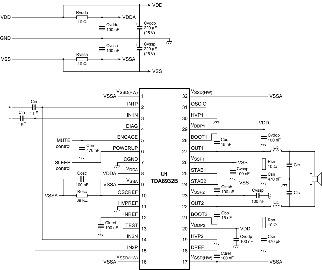
Fig 39. Typical simplified application diagram for 1 × BTL (symmetrical supply)
