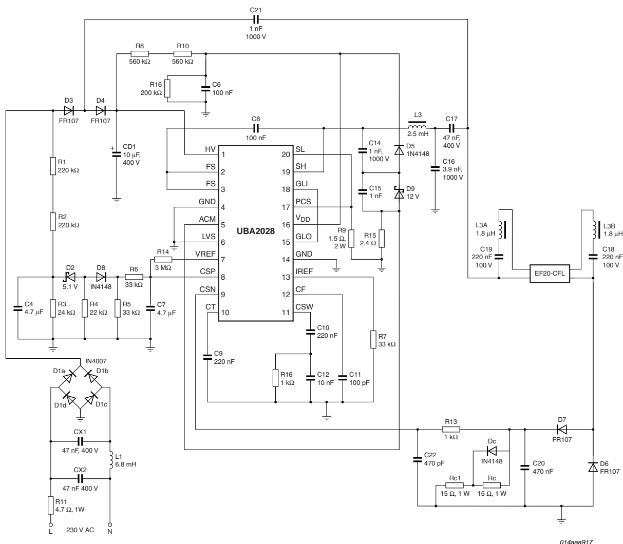
Fig 9. Application circuit 230 V
