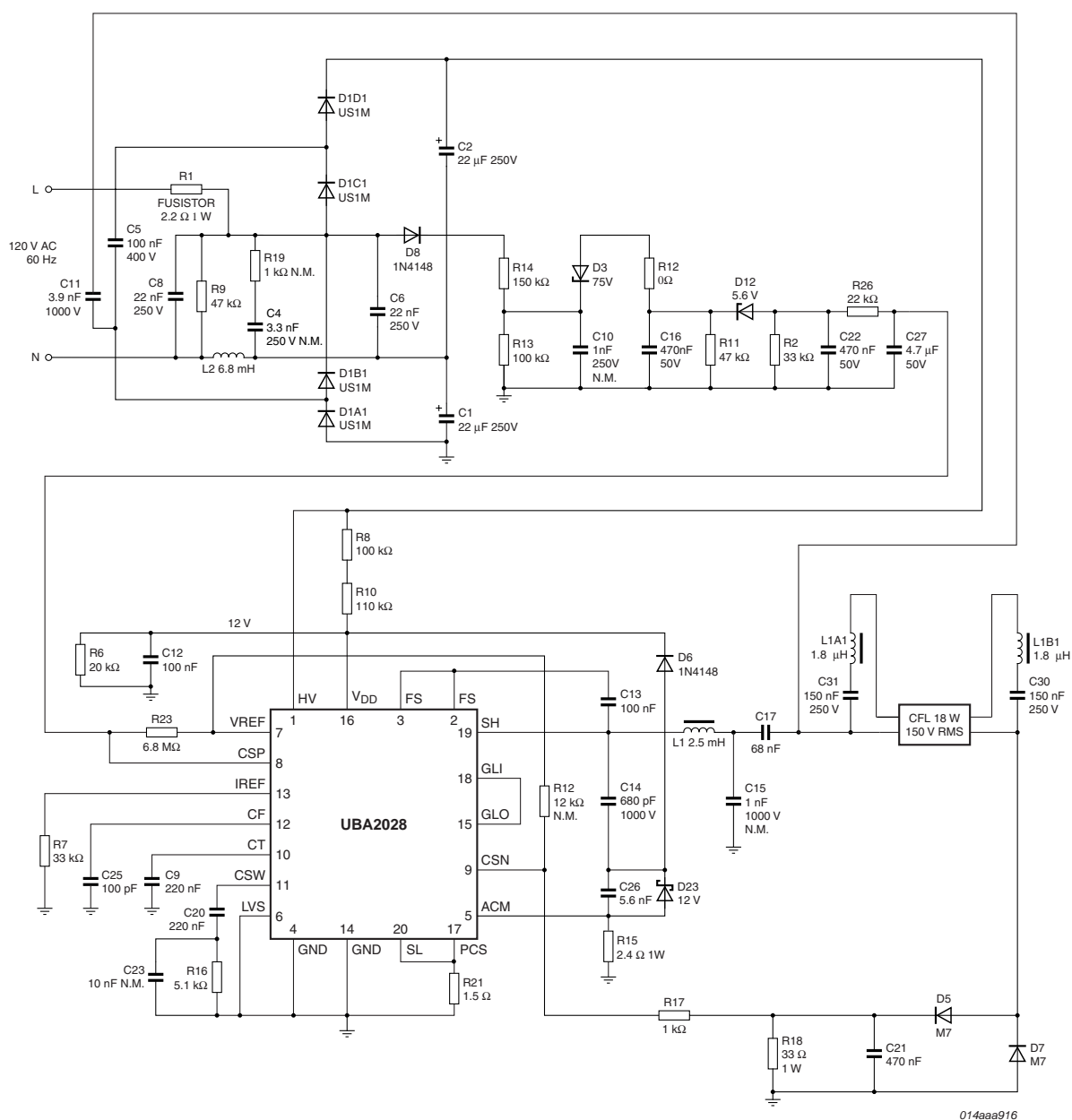
Fig 8. Application circuit 120 V
