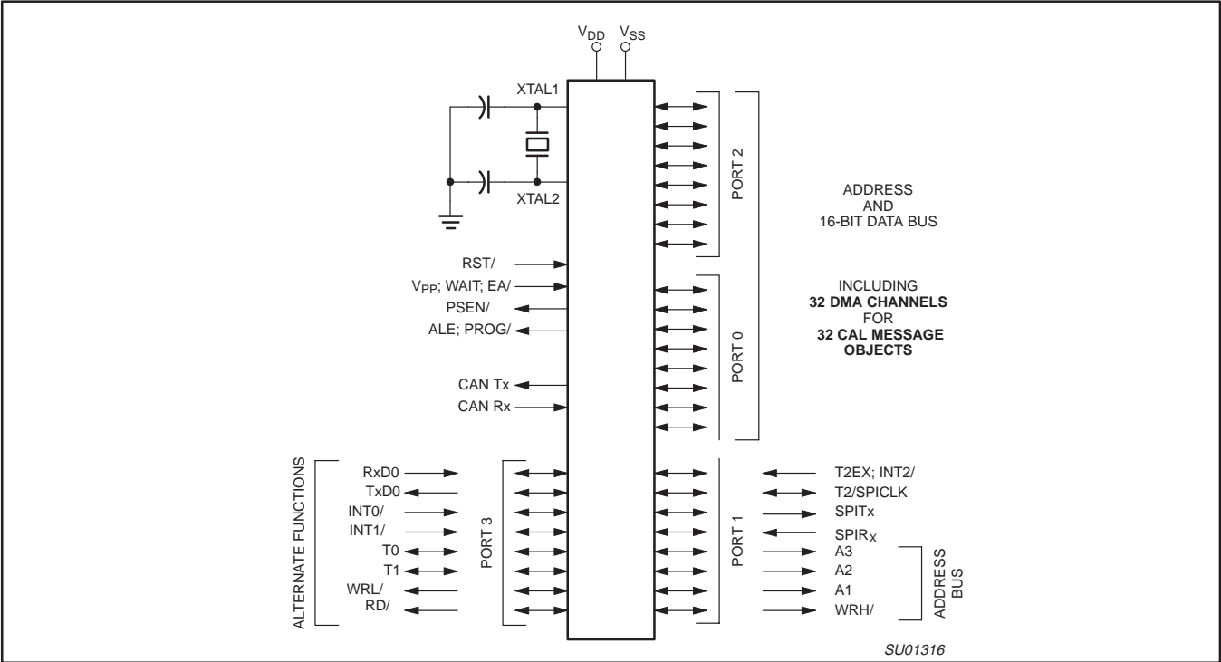
Figure 3. Logic Symbol
