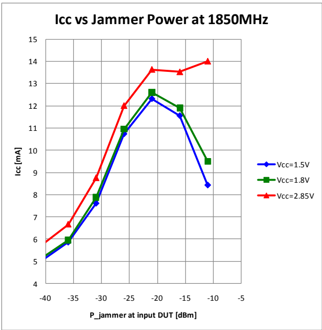
Fig 13. I CC versus jammer power
