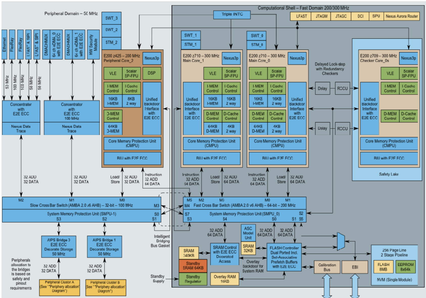
Figure 1. Block diagram
