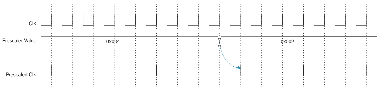
Figure 12-2. Prescaler Value Change Timing Diagram
