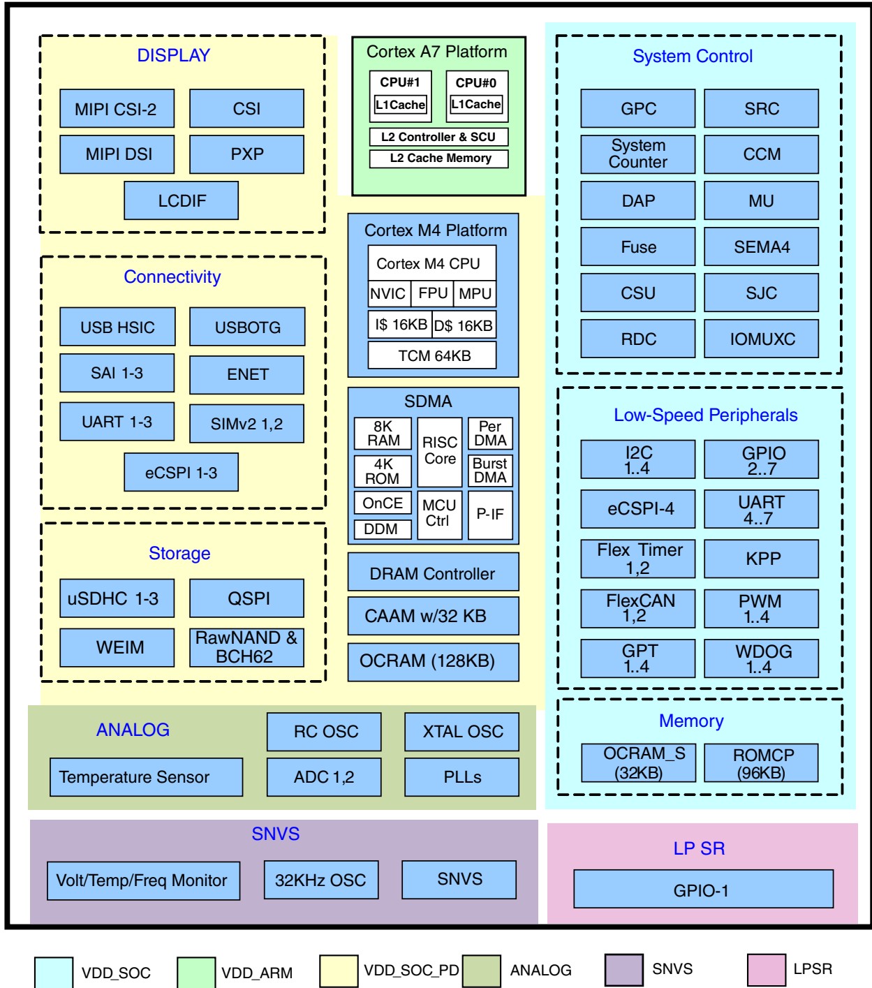
Figure 5-10. Power Domains
