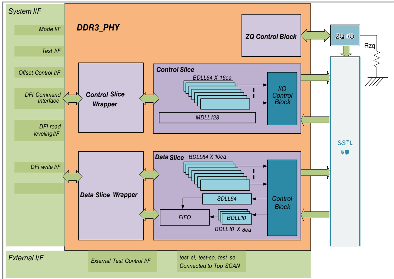
Figure 9-9. LPDDR3 HPHY
