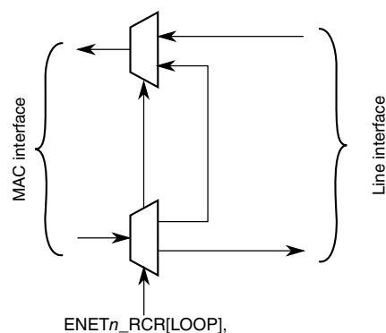
Figure 11-15. Loopback options
