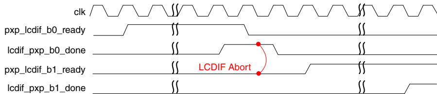
Figure 13-88. LCDIF Abort
