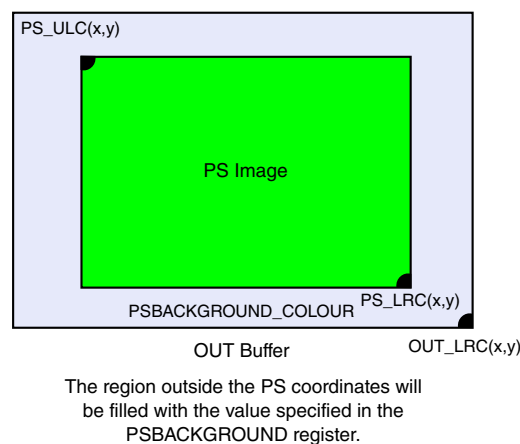
Figure 13-90. OUT Buffer
