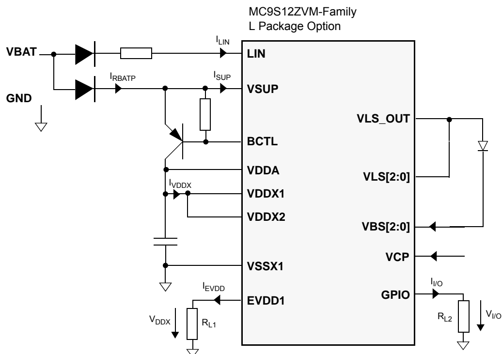
Figure A-2. Supply Currents Overview
