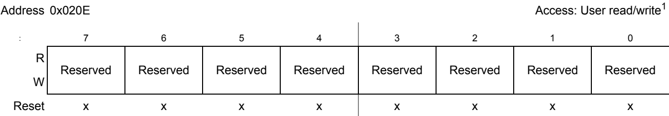
Figure 2-10. Reserved Register
