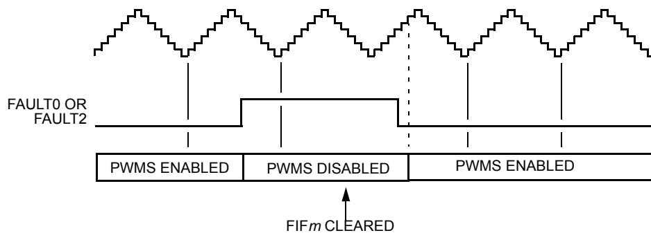
Figure 15-84. Manual Fault Recovery (Faults 0 and 2) — \text{QSMP} = 00
