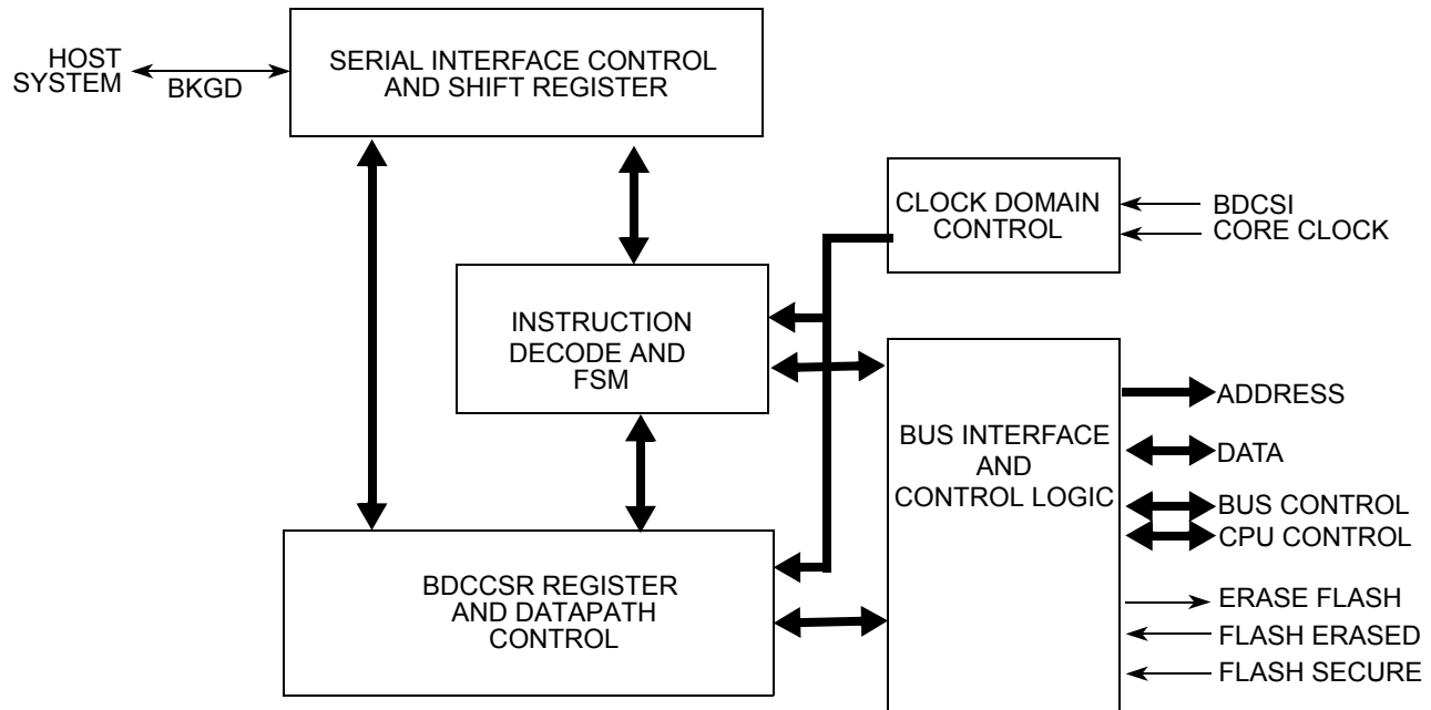
Figure 5-1. BDC Block Diagram
