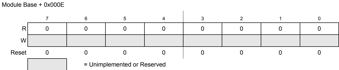
Figure 8-19. Reserved Register (CPMUTEST1)
