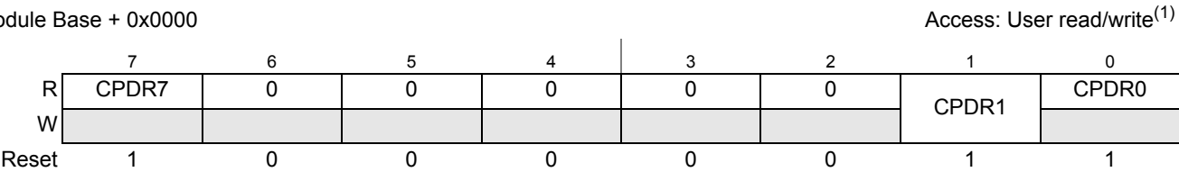
Figure 21-2. Port CP Data Register (CPDR)
