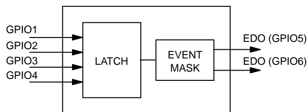
Figure 84. EDO Circuit
