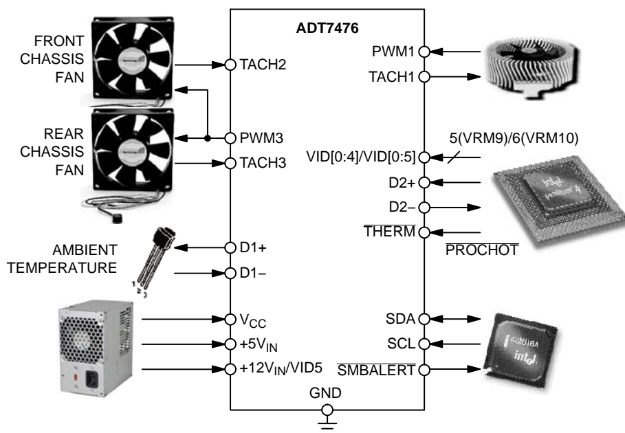
Figure 13. ADT7476 Configuration
