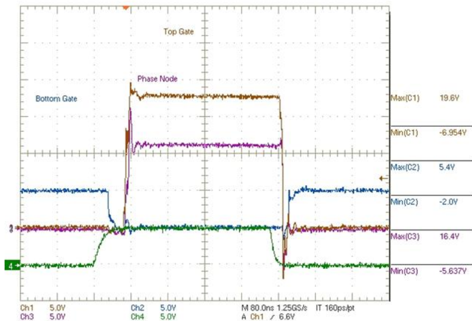
Figure 10: PWM Signal at G1 for I_{out} = 20A
