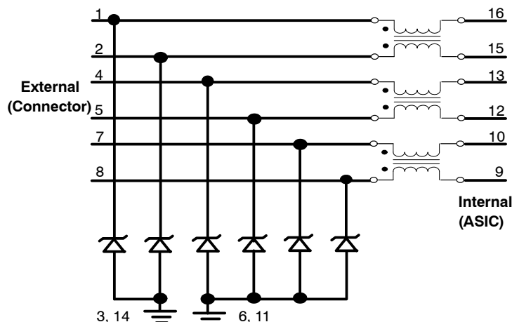
Figure 1. EMI4163MU Electrical Schematic
