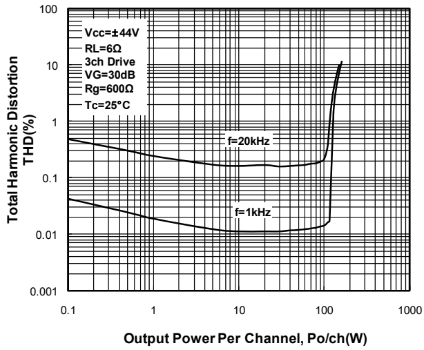
THD-Po STK433-330N-E
